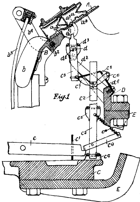
20892 Thomas. Linotype Machine. (Scharf.)
