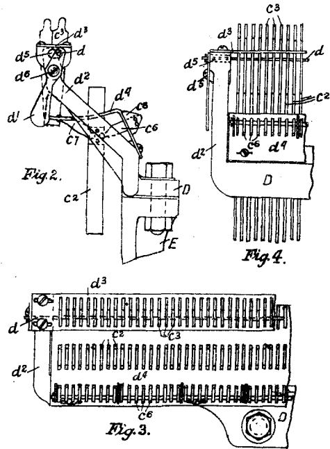
20892 Thomas. Linotype Machine. (Scharf.)
