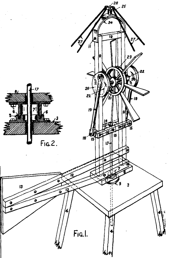
20973 McMaster. Windmill.
